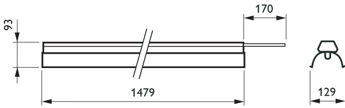
TTX261/262/263 1 x TL5 C-DA
