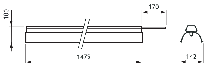
TTX261/262/263 1 x TL5 C-WB/CP-WB
